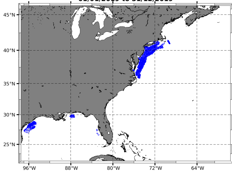
HFR-US-EastGulfCoast: HFR Surface current average [m/s] 01/01/2019 to 31/12/2019
