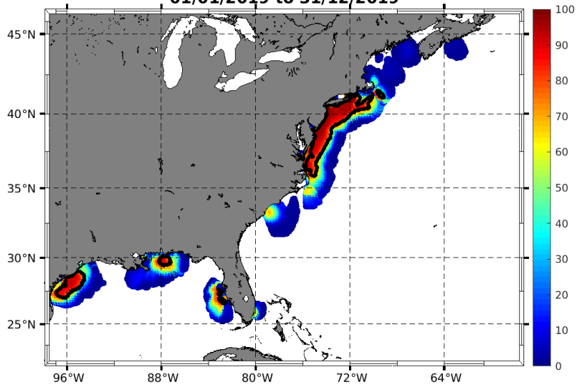
-US-EastGulfCoast: Percent Total Vector Coverage (contour showing >80% 01/01/2019 to 31/12/2019
